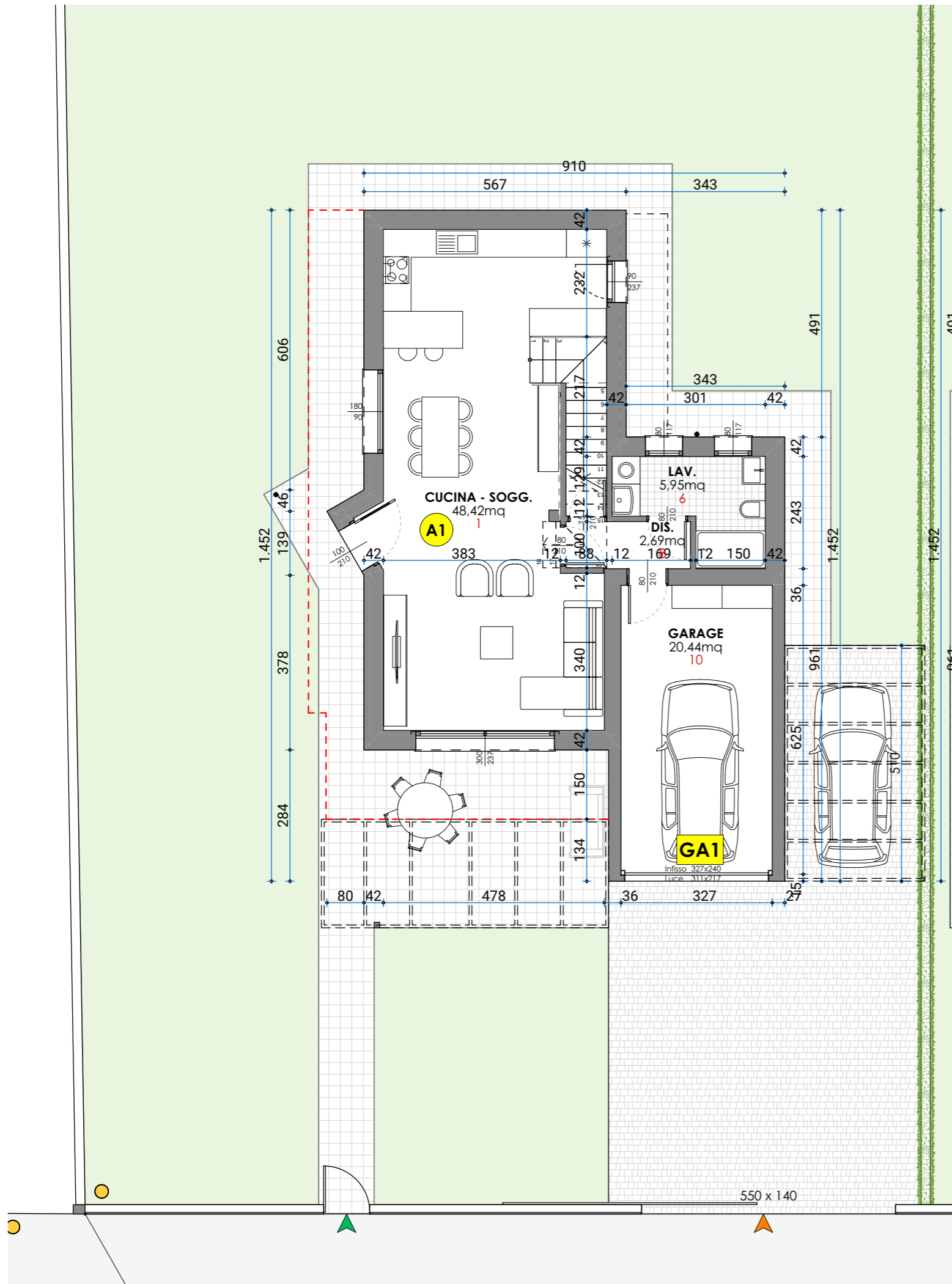
0. PIANO TERRA 1:100
